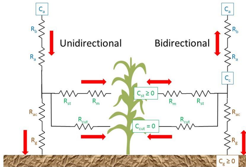
Figure 4-5. Right side shows a schematic of the bidirectional NH 3 deposition/re-emission scheme of Zhang et al. (2010) and Whaley et al. (2018); left side shows the original unidirectional deposition scheme of Zhang et al. (2003). Pathway resistances (R) and bidirectional compensation points (C) are shown.
