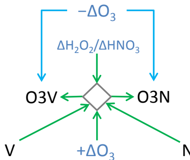
Figure 7-4. The OSAT2 scheme for ozone apportionment. Information flows along arrows. Changes in core model species are shown in blue, OSAT tracers are in black, the diamond represents the OSAT algorithm that determines ozone tracer production. \Delta H_2O_2 / \Delta HNO_3 is the indicator ratio used to determine NO x - or VOC-limited ozone production.
