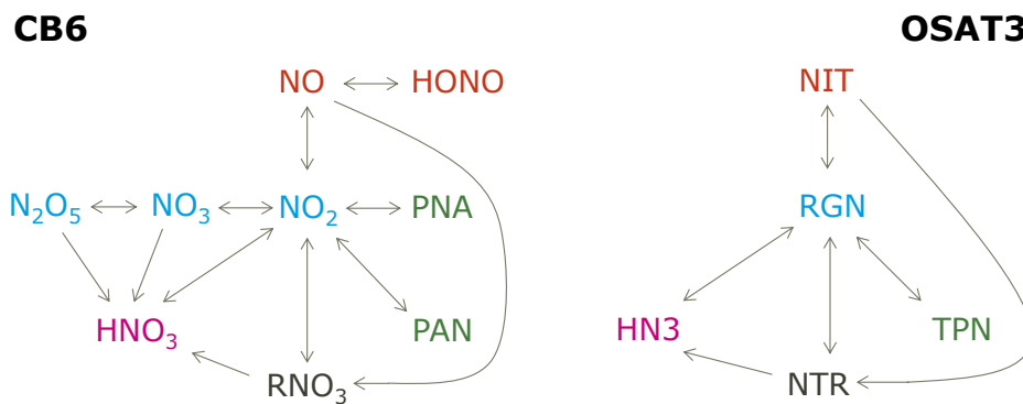
Figure 7-5. Correspondence between NO y species in CB6 and tracer families in OSAT3 with conversions between species/tracers shown by arrows.
