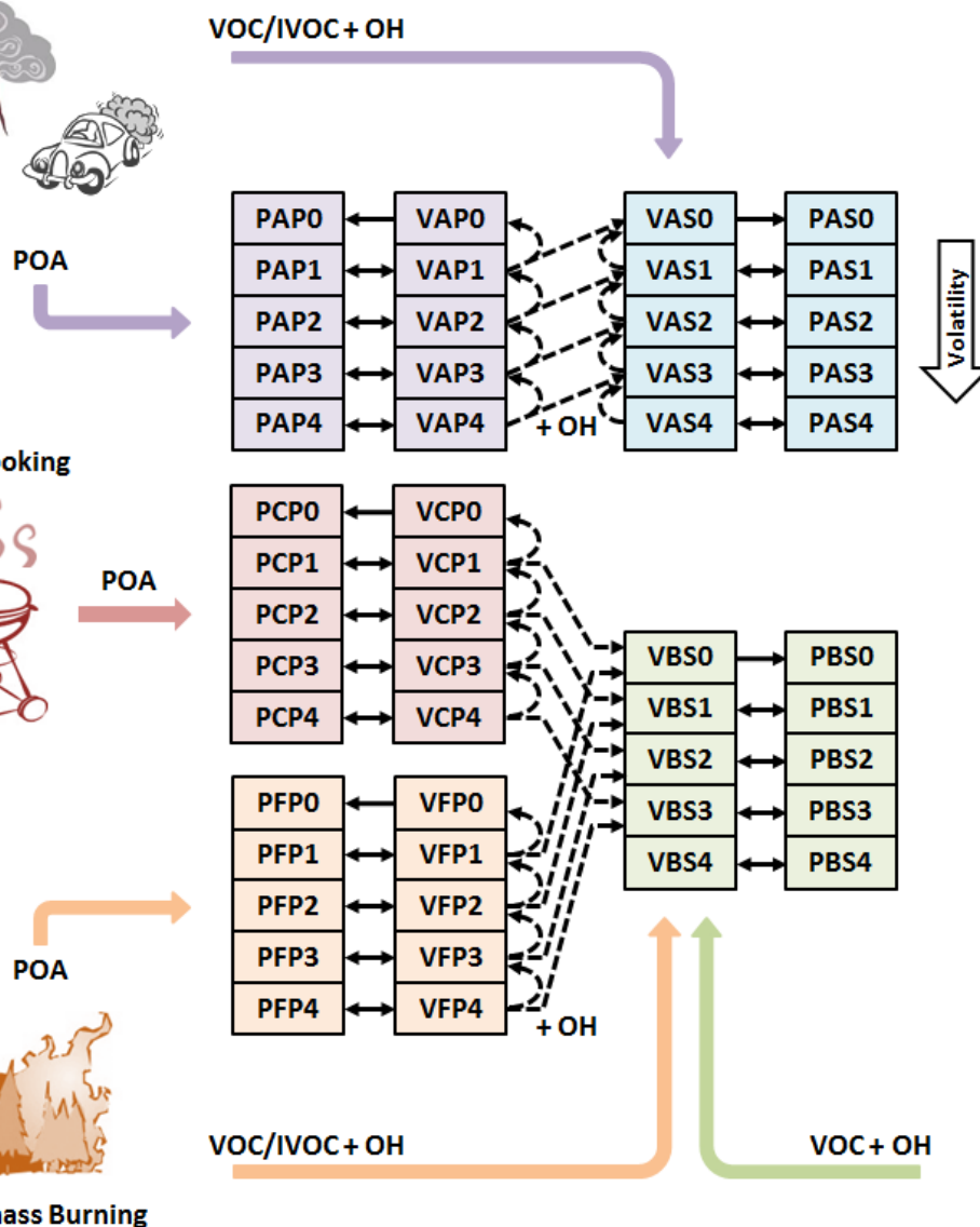
Figure 5-2. Schematic diagram of the CAMx VBS module. The model VBS species name consists of 4 characters that indicate the phase (P – particle; V – vapor), the source (A – anthropogenic; B – biogenic; C – cooking; F – fire), the formation (P – primary; S – secondary), and the volatility bin number. The solid and dashed arrows represent gas-aerosol partitioning and chemical aging, respectively. The thick colored arrows represent POA emissions or oxidation of SOA precursors.
