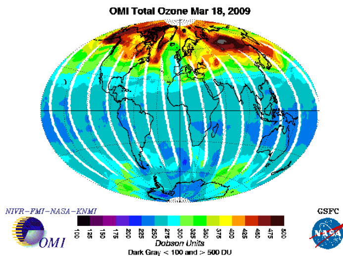
Figure 2-4. An example of global ozone column from the Ozone Monitoring Instrument (OMI) platform. White areas denote missing data. From ftp://toms.gsfc.nasa.gov/pub/omi/data/ .
