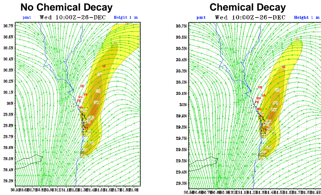
Figure 5-3. Impact of chemical decay on the concentration of the donor species PM2.5.
