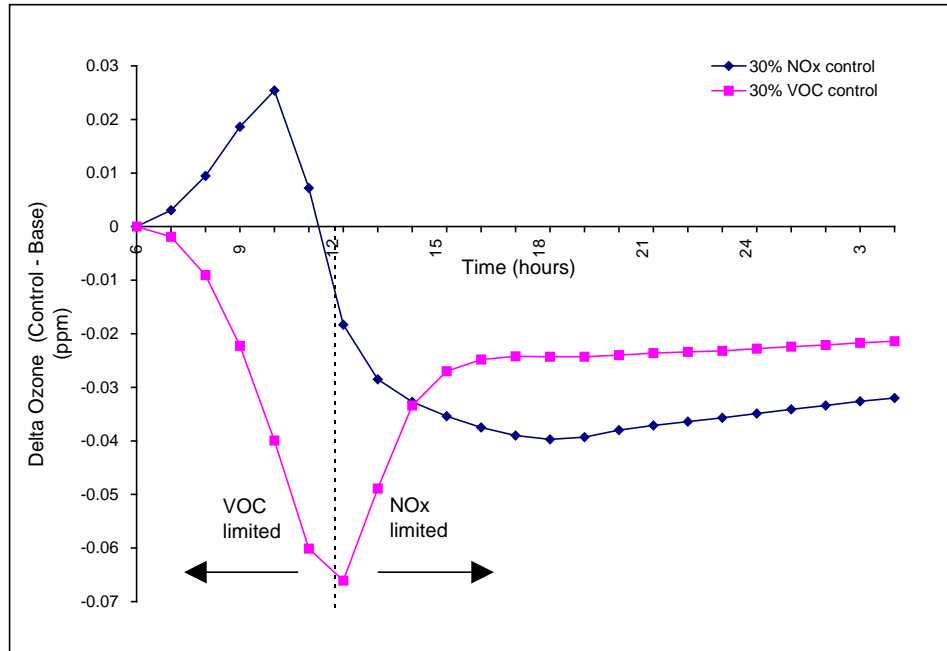
Figure 7-6. Change in ozone (control-base) for the VOC and NO x control scenarios shown in Figure 7-5. The vertical dashed line shows the transition from VOC to NO x limited ozone formation for the base case derived in Figure 7-4. Initial base case VOC/NO x = 10:1.
