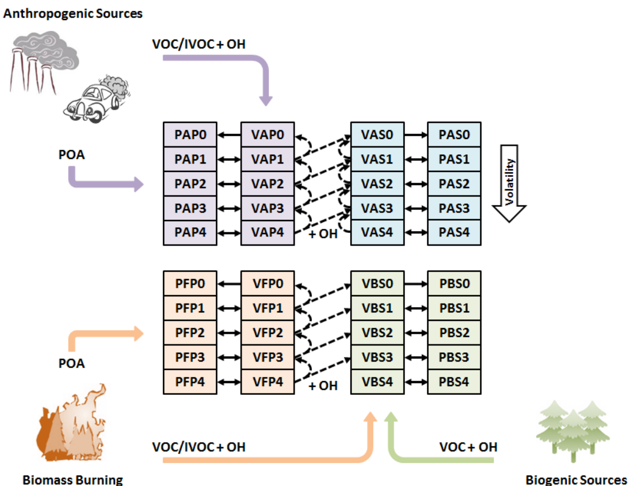
Figure 5-2. Schematic diagram of the CAMx VBS module. The model VBS species name consists of 4 characters that indicate the phase (P – particle; V – vapor), the source (A – anthropogenic; B – biogenic; F – fire), the formation (P – primary; S – secondary), and the volatility bin number. The solid and dashed arrows represent gas-aerosol partitioning and chemical aging, respectively. The thick colored arrows represent POA emissions or oxidation of SOA precursors.
