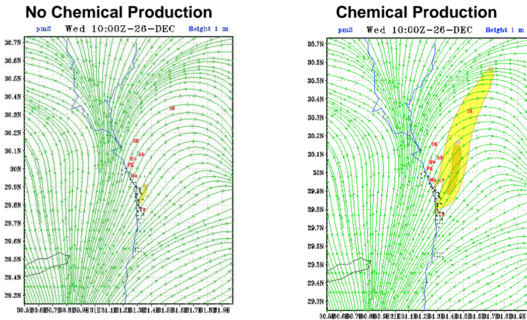
Figure 5-4. Impact of chemical production on the concentration of the recipient species PM2.5.
