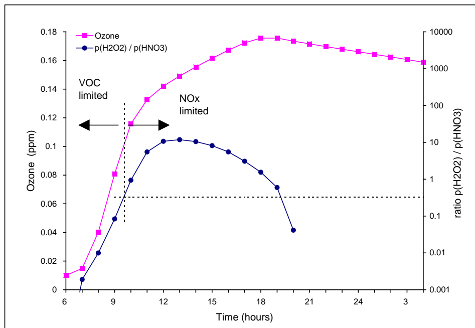
Figure 7-7a. As Figure 7-4, but for an Initial VOC/NO x = 20:1.
